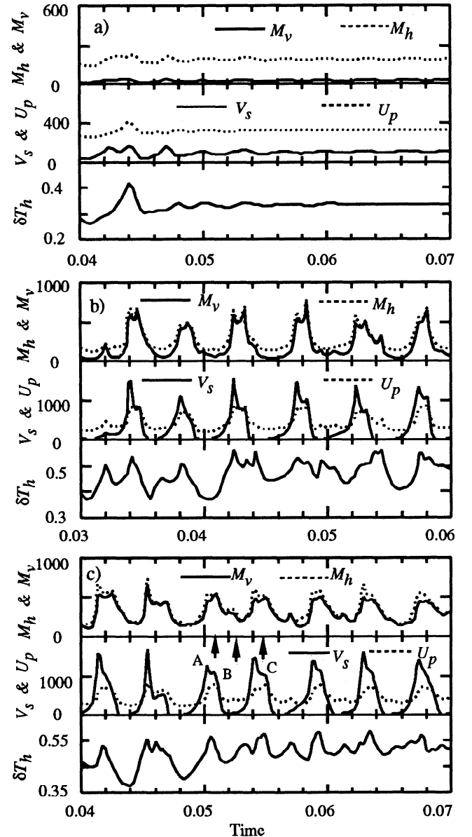
Figure 8. Time history of M_v , M_h , V_s , U_p , and \delta T_h for cases with an endothermic phase change, internal heating, and a plate of different length: (a) case 15 with L=1 , (b) case 16 with L=2 , and (c) case 17 with L=3 .
