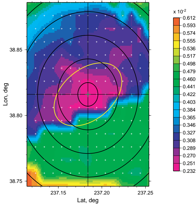
Figure 11: Residual/misfit surface for Event 13 showing the best fit location and error ellipse. Misfit between the Composite EGFs and the earthquake envelope functions. Black cross-hairs intersect at the GT location, the green plus sign marks the best fit location, coincident here with the GT location. Smaller white plus signs mark the \sim 1 km grid of hypothetical locations. Black contours denote distances of 1 km, 3 km, 5 km, etc from the GT location. The yellow error ellipse is the estimate for our location.
