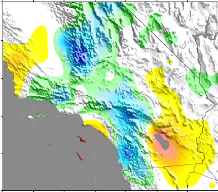
Receiver Functions
