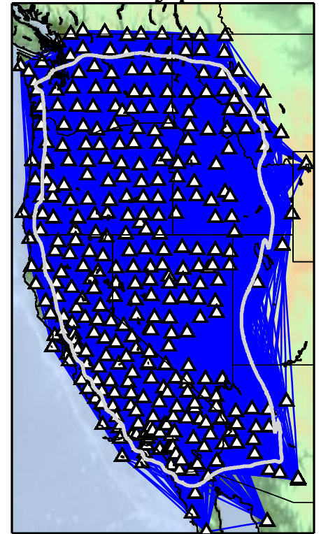
29608 ray paths
