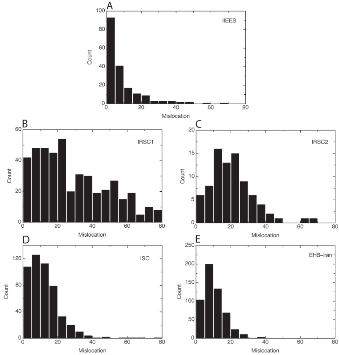
Figure 3. Histograms of mislocation distances of the different catalogs relative to the GT5 data set.
