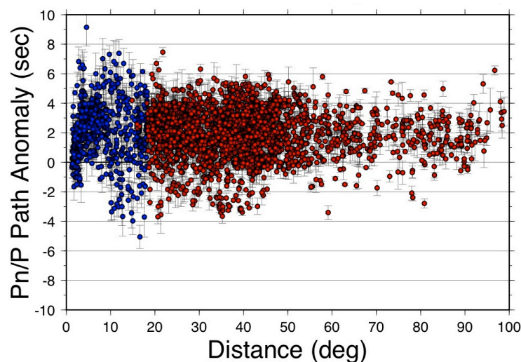
Figure 5. Empirical path anomalies for Pn (blue) and P (red) phases for GT5 90 events in the study region, calculated as the difference between the observed travel time of the phase arrival from a calibrated location (including origin time) and the theoretical travel time calculated with the ak135 velocity model. On average over the entire epicentral distance range, ak135-derived travel times are about 2 seconds faster than the travel times derived from calibrated locations.
