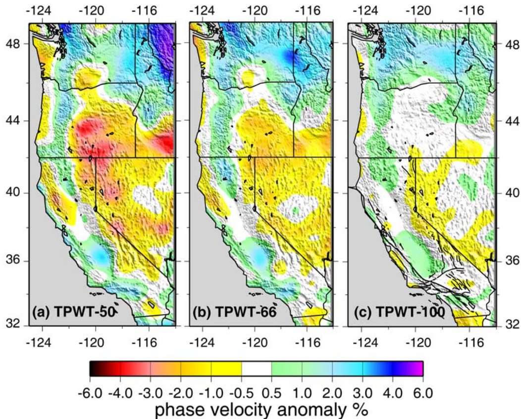
Figure 4. Rayleigh wave phase velocity maps from teleseismic two-plane wave tomography (TPWT) at periods of 50 (a), 66 (b) and 100 sec (c).
