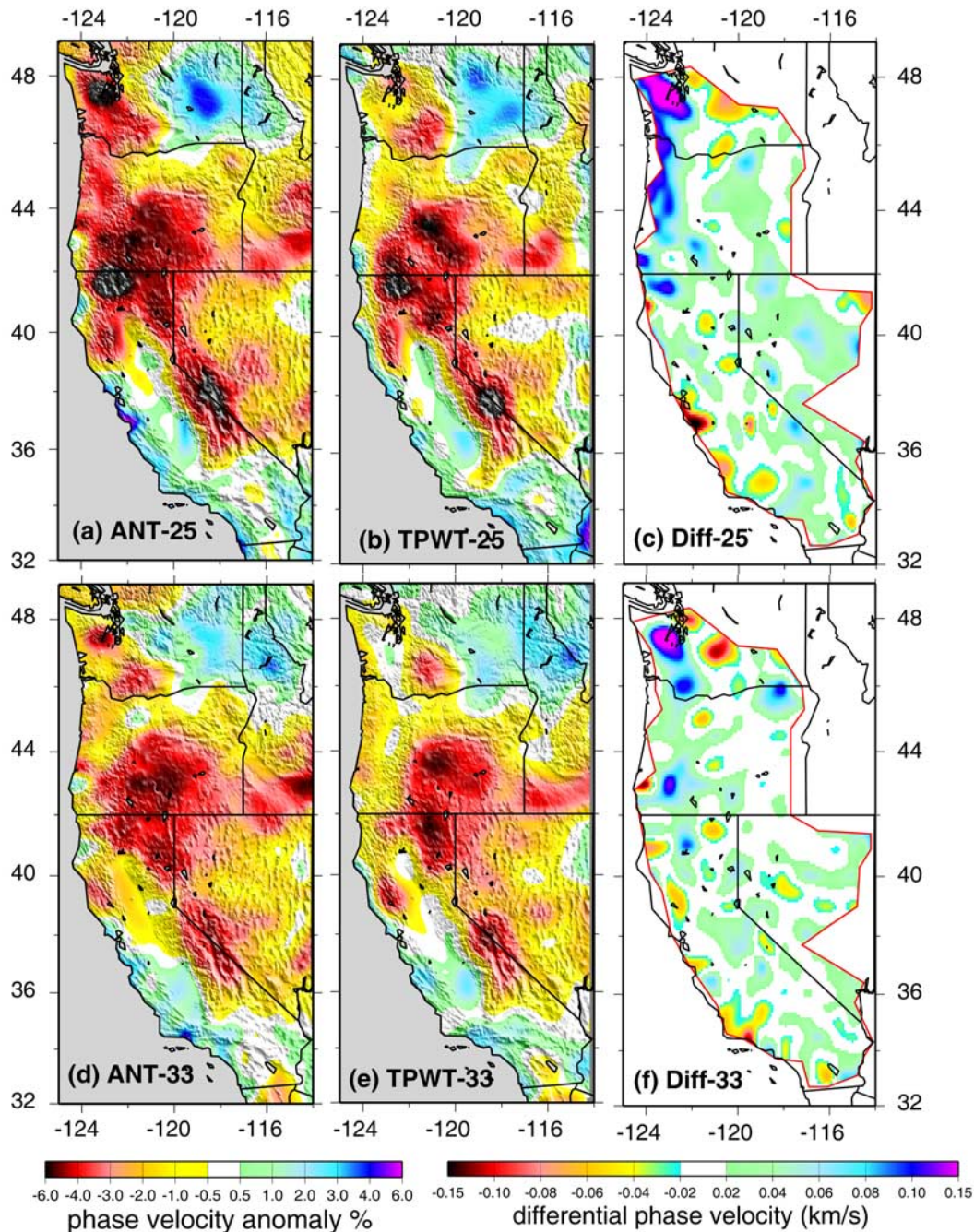
Figure 3. Rayleigh wave phase velocity maps from ambient noise tomography (ANT) compared with teleseismic two-plane wave tomography (TPWT). (a and b) ANT and TPWT at 25 s period, respectively. (d and e) ANT and TPWT at 33 s period, respectively. Anomalies are presented as the percent deviation from the average velocity across Southern California determined by Yang and Forsyth [2006a]. (c and f) Phase velocity differences between ANT and TPWT at 25 and 33 sec. The difference maps are clipped such that the red contour encompasses the region where seismic stations were deployed before September 15, 2006.
