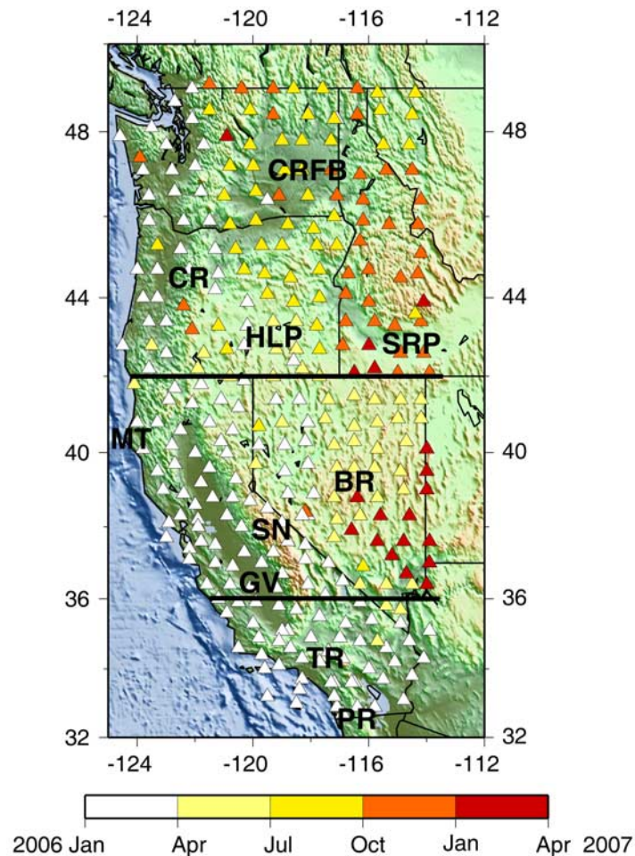
Figure 1. Station coverage and identification of the principal features of the western United States, including the Cascade Range (CR), the Columbia River Flood Basalts (CRFB), the High Lava Plain (HLP), the Snake River Plain (SRP), the Great Valley (GV), the Sierra Nevada Range (SN), the Basin and Range province (BR), the Transverse Range (TR) and the Peninsular Range (PR). Triangles mark the locations of the seismic stations used in this study, color coded by the first month we begin to collect teleseismic data in this study. The two bold lines divide the study region into three sub-regions: the Pacific-Northwest, northern California, and southern California. Teleseismic tomography is performed separately in each of the three sub-regions.
