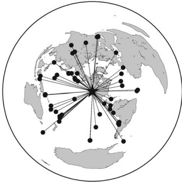
Figure 2. Azimuthal equidistant projection of teleseismic events (black circles) used in this study. The plot is centered at longitude -118^\circ and latitude 42^\circ as marked by the star. The straight lines connecting each event to the center are great-circle paths.
