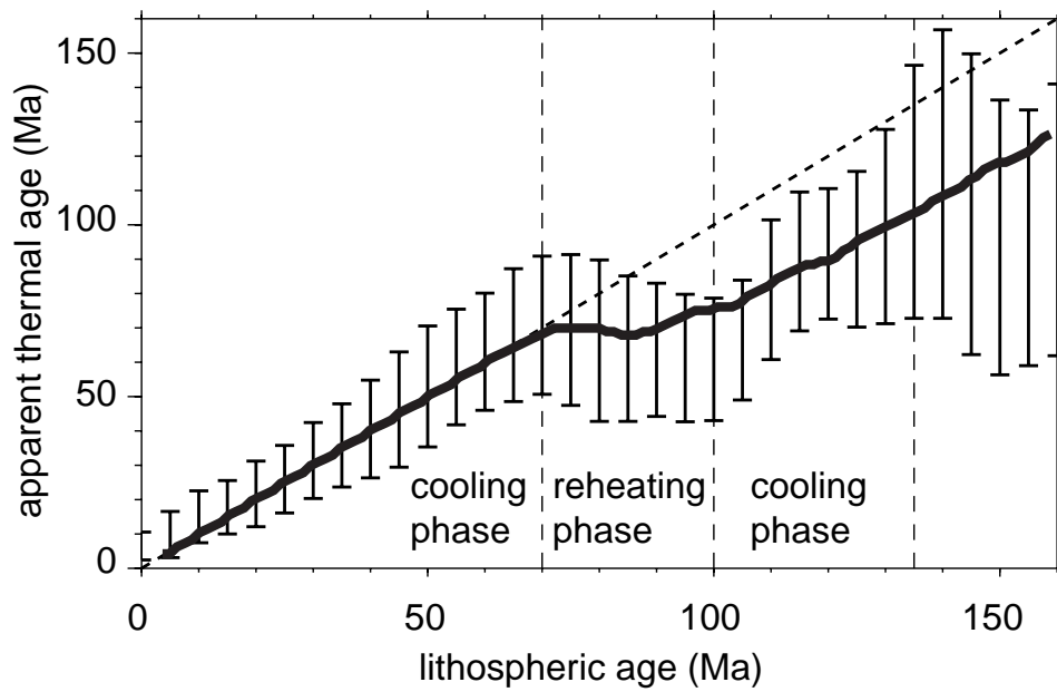
Figure 13: Simulation of TBI expressed as apparent thermal age versus lithospheric age. Similar to Figure 9a, except the thick black line is \tau , averaged in lithospheric age bins, computed from the 3-D convection model of thermal boundary layer instabilities, with an effective rheological activation energy of 120 kJ/mol.
