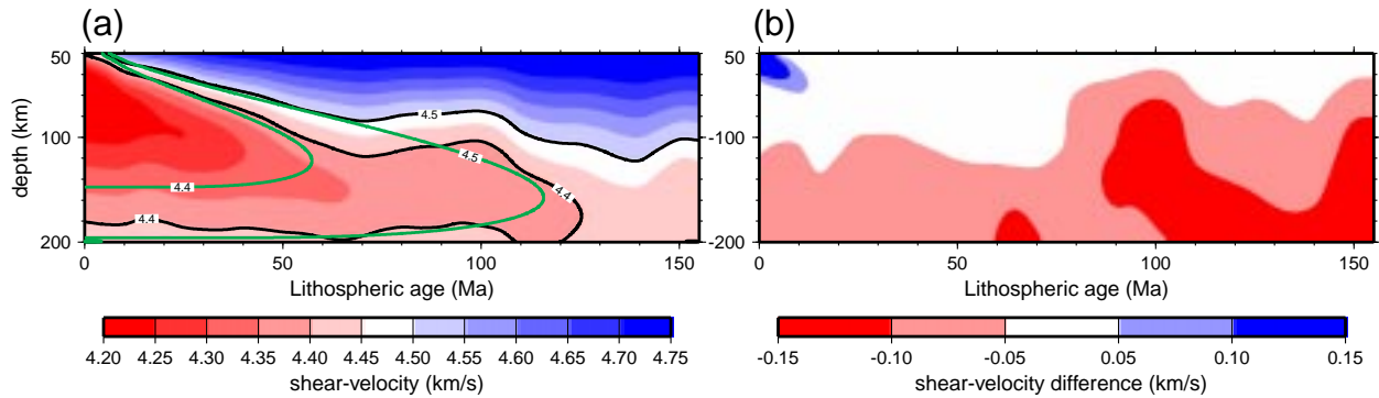
Figure 7: Shear velocity structure of the Pacific upper mantle and trend with lithospheric age using the thermal parameterization: Vertical profile. (a) V_s averaged across the Pacific plotted versus lithospheric age. The green lines are isotachs (lines of constant shear velocity) from the HSC model. (b) Difference between the Pacific average shear velocity and the prediction from the HSC model. Reds identify areas where the observed shear velocity is slower than the HSC model predicts.
