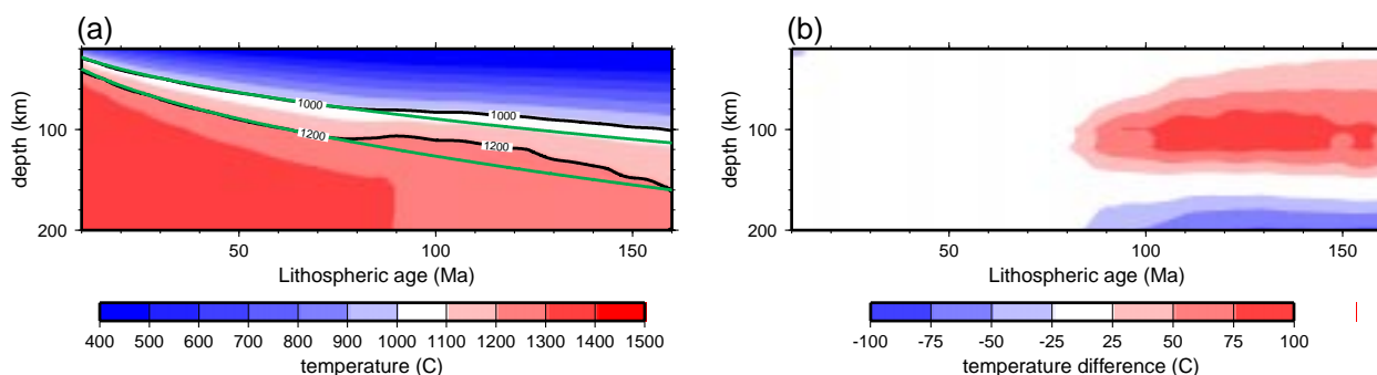
Figure 7: Thermal structure versus lithospheric age for the simulation of TBI. (a) Temperatures from the 3-D convection simulation of thermal boundary layer instabilities are averaged parallel to the ridge at each depth and plotted versus lithospheric age. The green lines are isotherms from the HSC model. (b) The difference between the temperatures from the simulation of TBI with the HSC model. Reds imply that temperatures in TBI simulation are warmer than in the HSC model.
