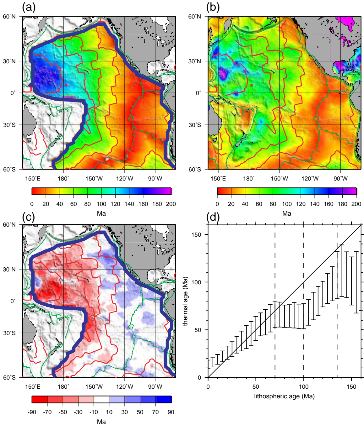
Figure 5: Thermal age and age trend determined with the seismic parameterization. (a) Lithospheric age in Ma, presented as a reference 1 . (b) Apparent thermal age, \tau , estimated with the seismic parameterization. (c) Difference between the lithospheric age and the apparent thermal age. Reds denote that the apparent thermal age is younger than the lithospheric age. In (a) and (b), the green, red, and blue lines are as in Figure 2a-2f. (d) Comparison between apparent thermal age and lithospheric age. Apparent thermal age is averaged in 5 Ma lithospheric age bins across the Pacific and error bars represent the standard deviation within each age range. Contrast with Figures 3 and 4 in the main text, based on the thermal parameterization.
